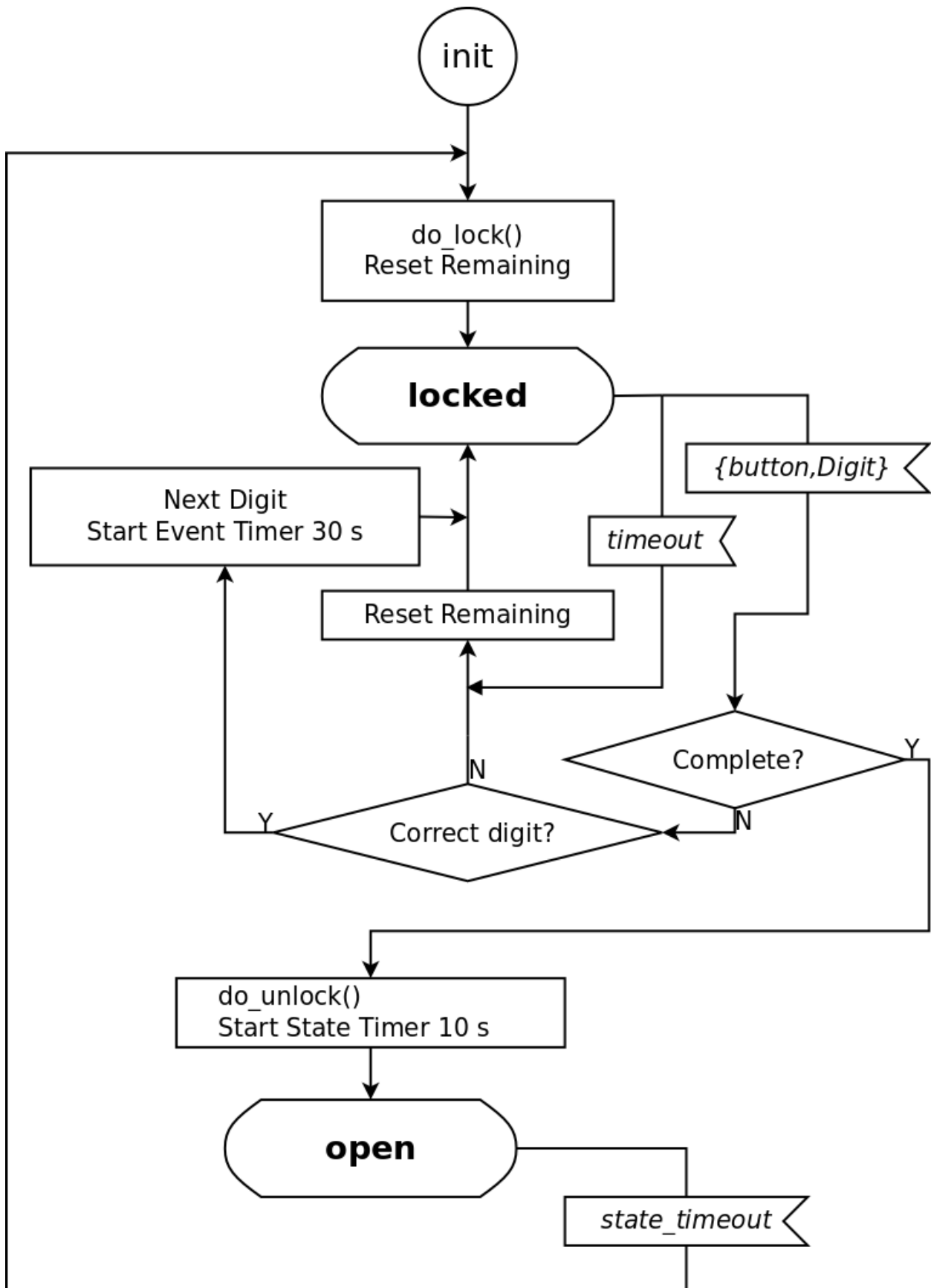
Figure 3.2: Code Lock State Diagram Revisited. Ericsson AB. All Rights Reserved.: Erlang/OTP System Documentation | 299
